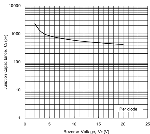
Fig. 5 - Junction Capacitance
