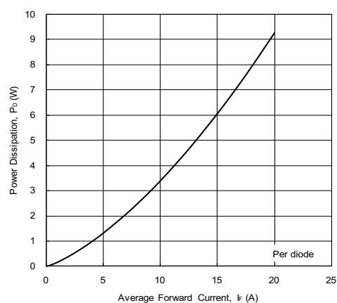
Fig. 4 - Forward Power Dissipation
