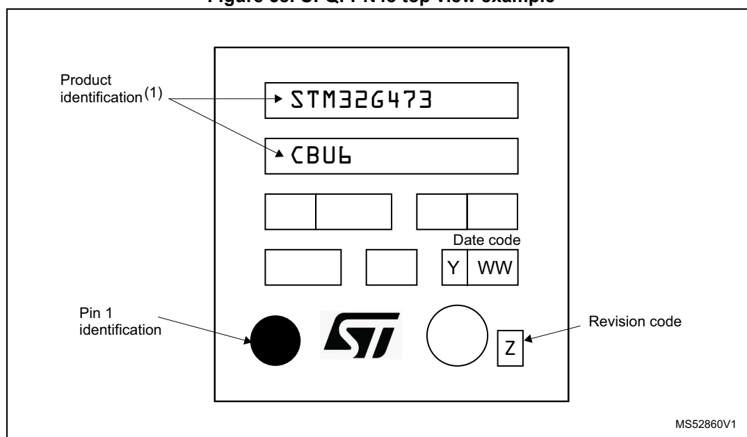
Figure 58. UFQFPN48 top view example
