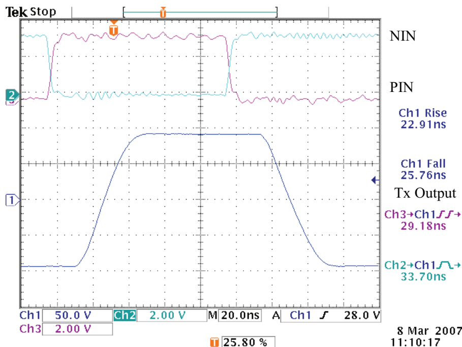
Figure 2: Input to output propagation delay on rise is 29ns and on fall is 33.7ns and the tr/tf time is 22.9/25.8ns V_{LL} = 3.3V , V_{DD} = +10V , (V_{PP} - V_{PF}) = +10V , (V_{NF} - V_{NN}) = +10V , V_{PP}/V_{NN} = +/-90V , V_{SUB} = +95V with load of 330pF//2.5K, at MC0 = MC1 = 1.
