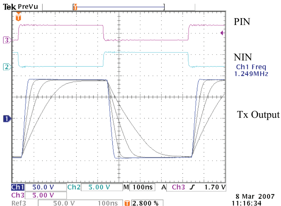
Figure 3: PIN, NIN and OUTPUT at 1.25MHz, V_{DD} = +10V , (V_{PP} - V_{PF}) = +10V , (V_{NF} - V_{NN}) = +10V , V_{PP}/V_{NN} = +/-90V , V_{SUB} = +95V with load of 330pF//2.5K \Omega , Load = 330pF//2.49k \Omega , Mode 1 through 4 current modes.
