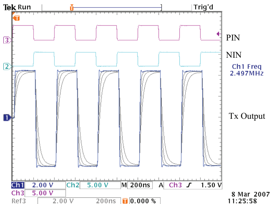
Figure 4: PIN, NIN and OUTPUT at 2.5MHz, V_{DD} = +10V , (V_{PP} - V_{PF}) = +10V , (V_{NF} - V_{NN}) = +10V , V_{PP}/V_{NN} = +/-5.0V , V_{SUB} = +95V with load of 330pF//2.5K \Omega , Load = 330pF//2.49k \Omega , Mode 1 through 4 current modes.
