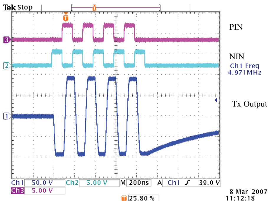
Figure 1: PIN, NIN and output waveform of 5MHz, V_{LL} = 3.3V , V_{DD} = +10V , (V_{PP} - V_{PF}) = +10V , (V_{NF} - V_{NN}) = +10V , V_{PP}/V_{NN} = +/-90V , V_{SUB} = +95V with load of 330pF//2.5K, at MC0 = MC1 = 1.
