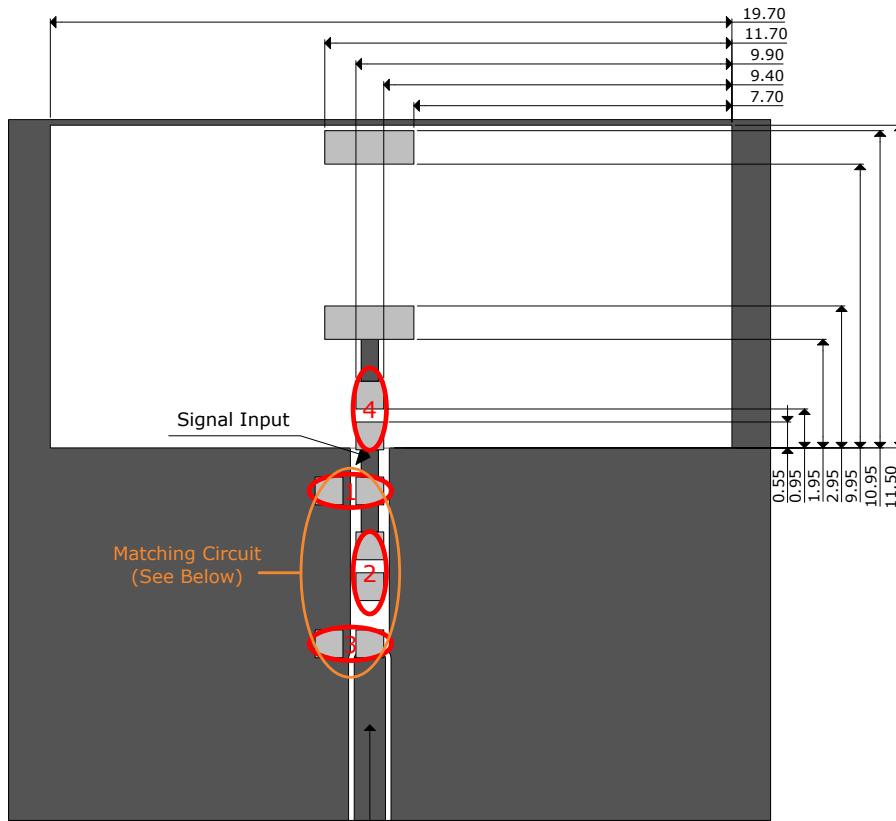
Transmission Line With 50Ω Impedance Characteristics
