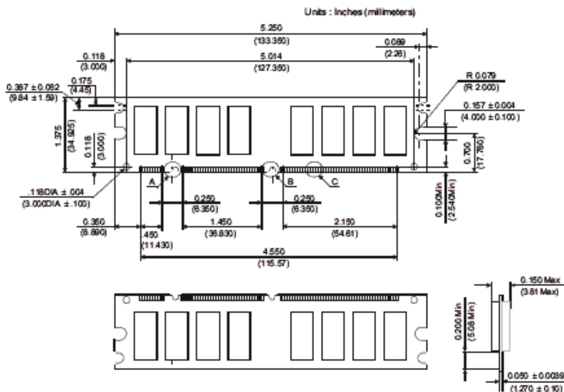
Figure 1: KVR100X64C2/128 168-Pin SDRAM Module
