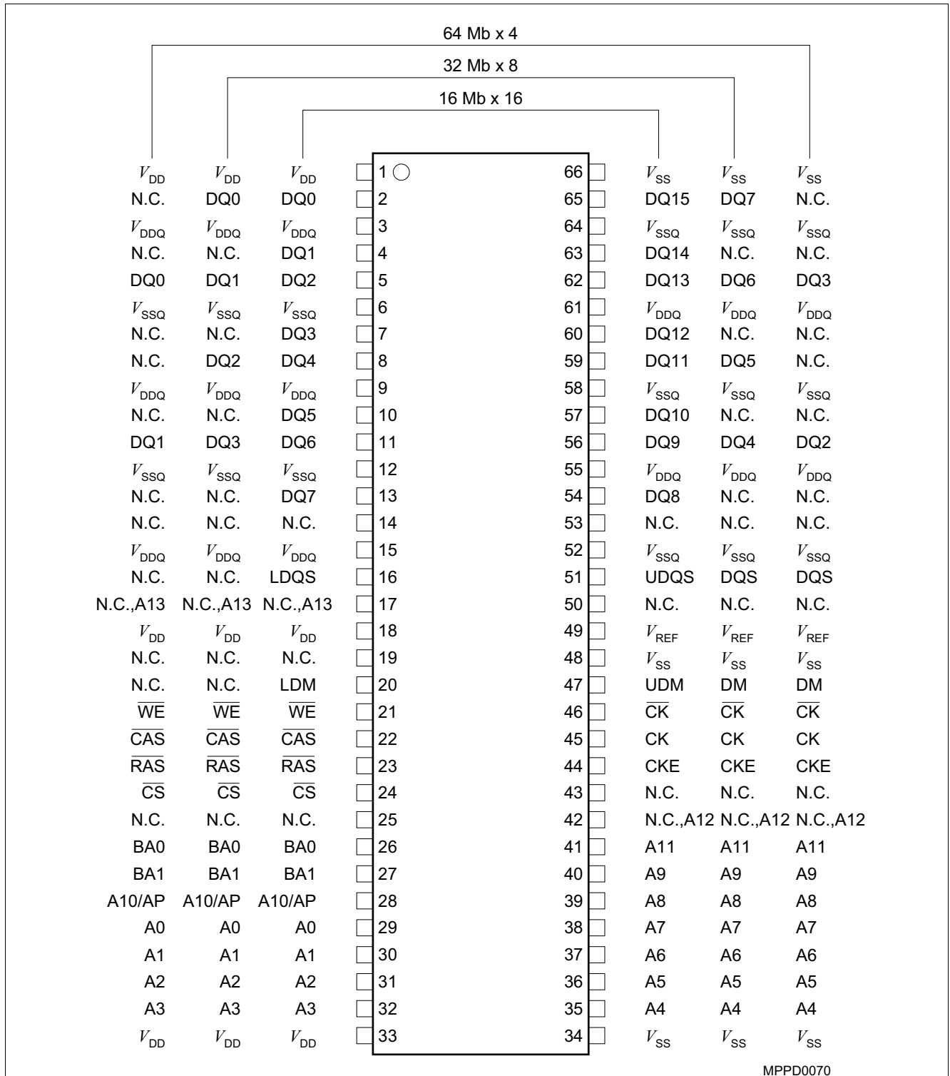
Figure 2 Pin Configuration P-TSOP11-66-1
