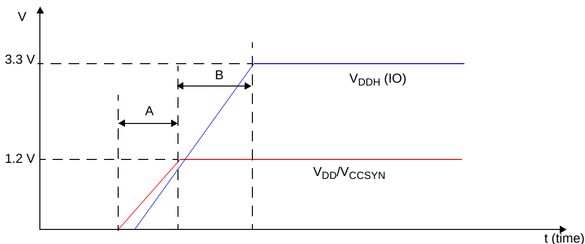
Figure 8. Power-Up Sequence for V_{\text{DDH}} and V_{\text{DD}}/V_{\text{CCSYN}}
