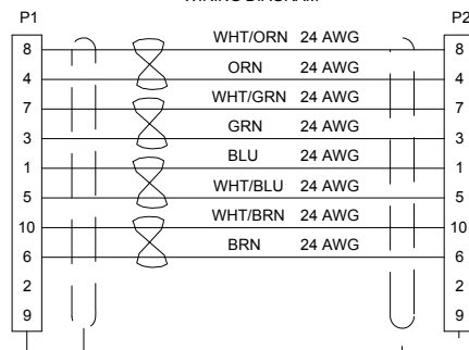
WIRING DIAGRAM
