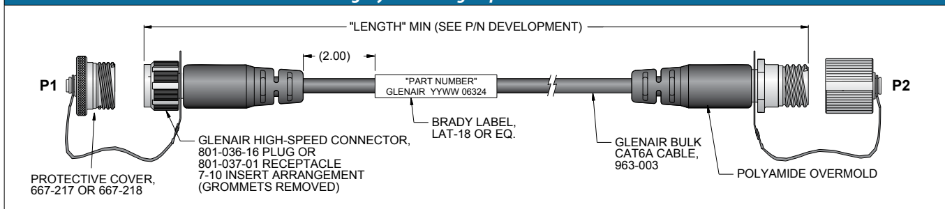
801-046: Series 801 Mighty Mouse High-Speed 10GBASE-T Overmolded Cordset
