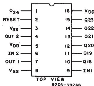
TERMINAL ASSIGNMENT
