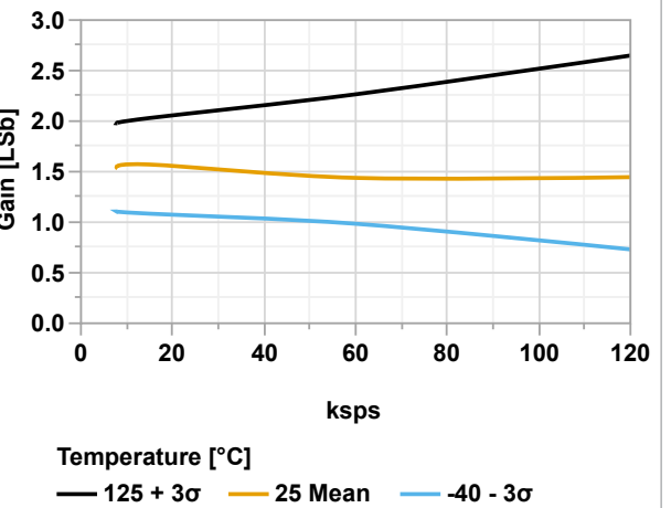
Figure 38-122. Positive Gain Error vs. Sample Rate (ADC Differential Mode, V_{\text{REFA}} = V_{\text{DD}} = 3.6\text{V} )
