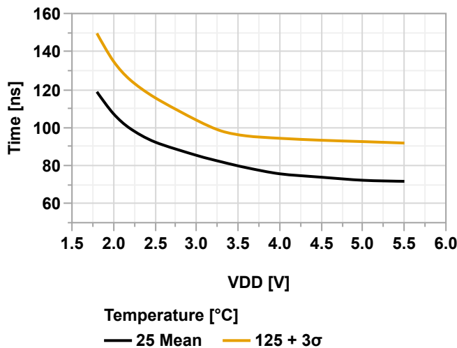
Figure 38-136. Falling Edge Response Time vs. V_{DD} ( V_{CM} = V_{DD}/2 , CTRLA.POWER = 0x00)
