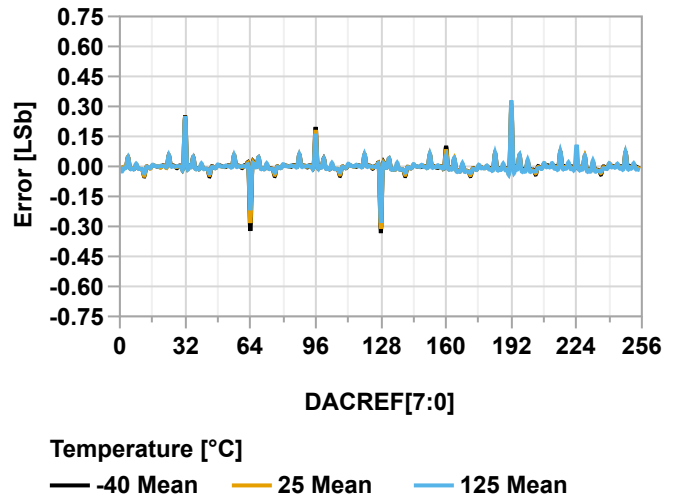
Figure 38-165. INL vs. DAC Code ( V_{\text{REFA}} = V_{\text{DD}} = 5.5\text{V} )
