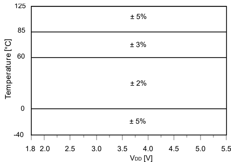
Figure 37-2. Precision Calibrated OSCHF (4 MHz) and OSC32K Frequency Accuracy Over Device V_{\text{DD}} and Temperature (1)
