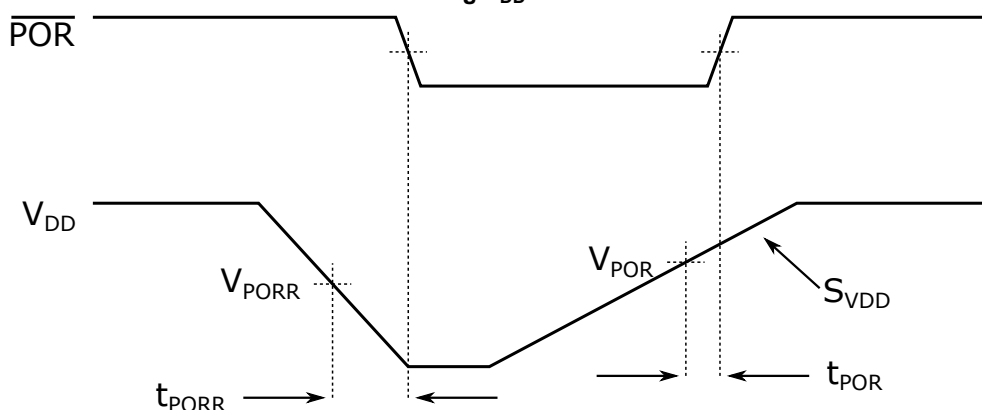
Figure 37-1. \overline{\text{POR}} and \text{POR} Re-Arm with Slow Rising V_{\text{DD}}
