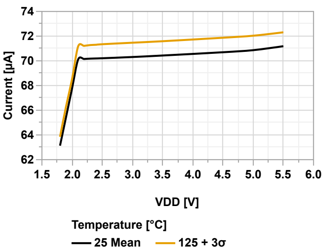
Figure 38-39. VREF Power Consumption vs. V_{DD} (ACREF Enabled)
