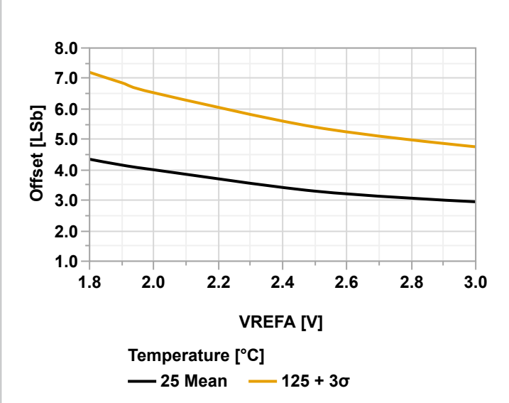
Figure 38-113. Offset Error vs. V_{\text{REFA}} (ADC Single Ended Mode @60 ksps, V_{\text{DD}} = 3.0\text{V} )
