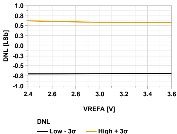
Figure 38-129. DNL vs. V_{\text{REFA}} (ADC Differential Mode @60 kps, V_{\text{DD}} = 3.6\text{V} , T = 85^\circ\text{C} )
