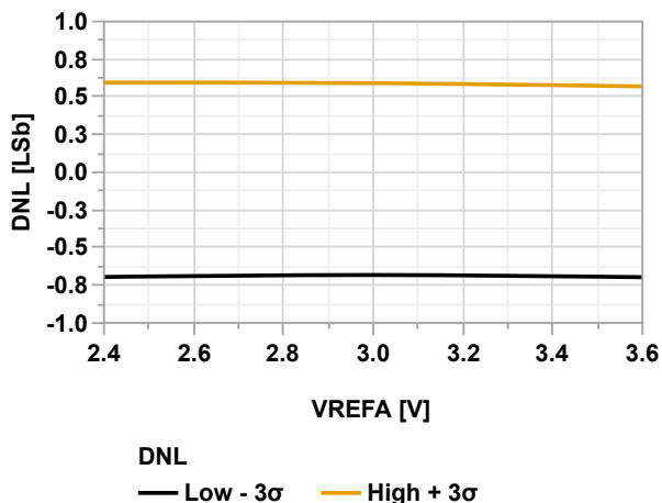
Figure 38-130. DNL vs. V_{\text{REFA}} (ADC Differential Mode @60 kps, V_{\text{DD}} = 3.6\text{V} , T = 125^\circ\text{C} )
