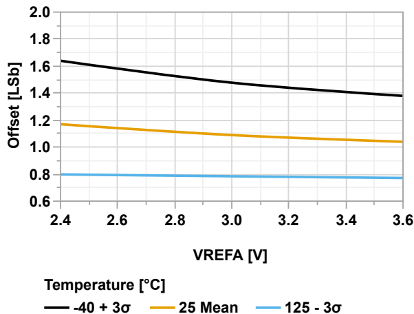
Figure 38-125. Offset Error vs. V_{\text{REFA}} (ADC Differential Mode @60 ksps, V_{\text{DD}} = 3.6\text{V} )
