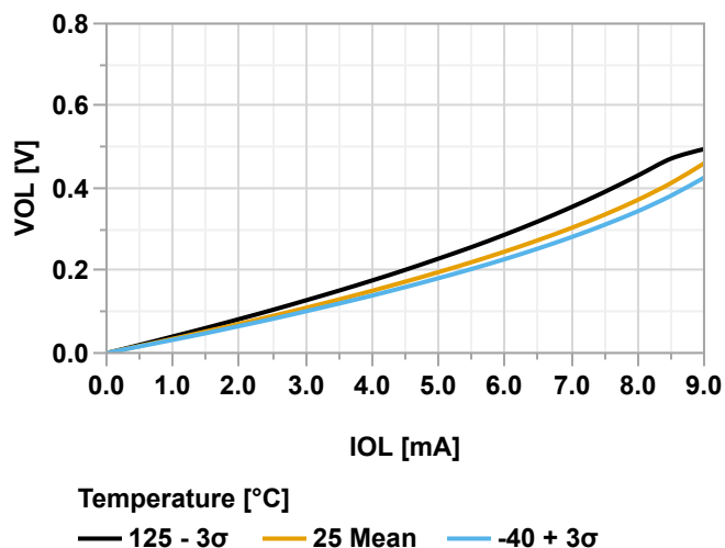
Figure 38-85. Output Pin - Maximum V_{OL} vs. Current, V_{DD} = 3.0V
