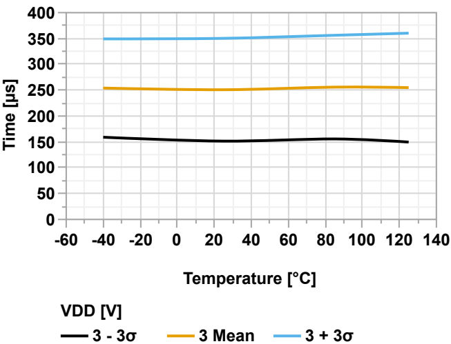
Figure 38-157. Settling Time vs. Temperature ( V_{\text{REFA}} = V_{\text{DD}} = 3.0\text{V} , Output Switch from 0x3FF to 0x000)
