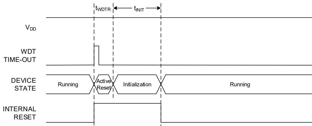
Figure 13-4. Watchdog Reset
