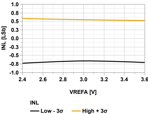
Figure 38-134. INL vs. V_{\text{REFA}} (ADC Differential Mode @60 kps, V_{\text{DD}} = 3.6\text{V} , T = 125^\circ\text{C} )
