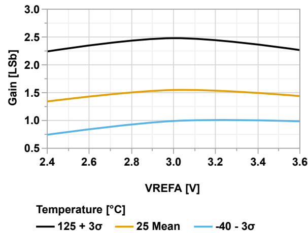
Figure 38-121. Positive Gain Error vs. V_{\text{REFA}} (ADC Differential Mode @60 kps, V_{\text{DD}} = 3.6\text{V} )
