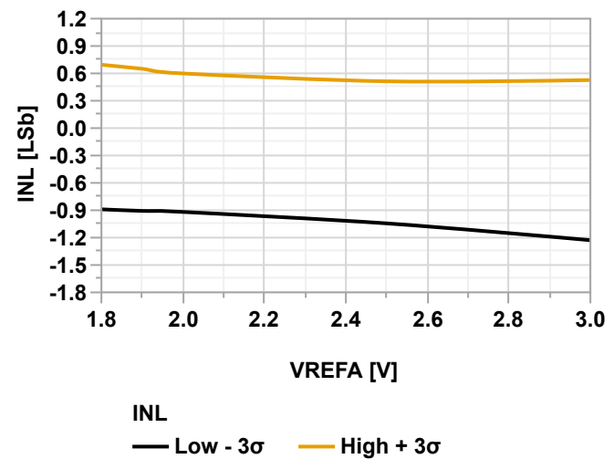
Figure 38-119. INL vs. V_{\text{REFA}} (ADC Single Ended Mode @60 kps, V_{\text{DD}} = 3.0\text{V} , T = 125^\circ\text{C} )
