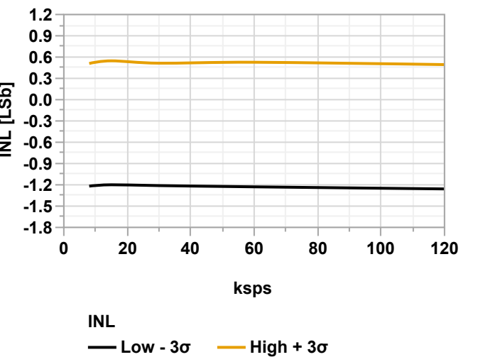
Figure 38-120. INL vs. Sample Rate (ADC Single Ended Mode, V_{\text{REFA}} = V_{\text{DD}} = 3.0\text{V} , T = 125^\circ\text{C} )
