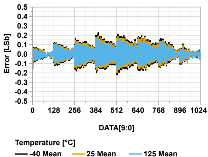
Figure 38-153. DNL vs. DAC Code ( V_{\text{REFA}} = V_{\text{DD}} = 5.5\text{V} )
