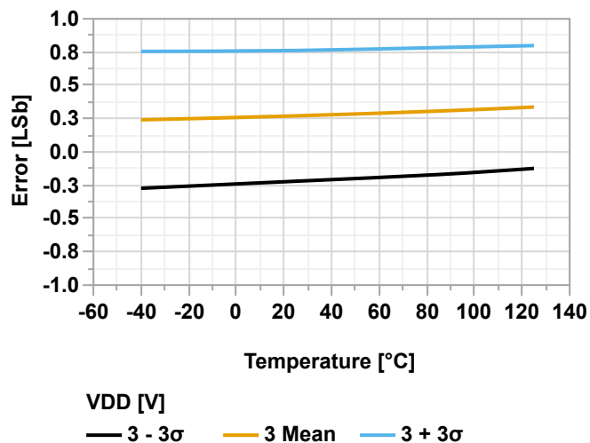
Figure 38-160. Offset Error vs. Temperature ( V_{\text{REFA}} = V_{\text{DD}} = 3.0\text{V} )
