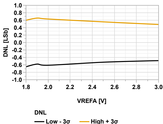
Figure 38-117. DNL vs. V_{REFA} (ADC Single Ended Mode @60 kps, V_{DD} = 3.0V , T = 125^{\circ}C )
