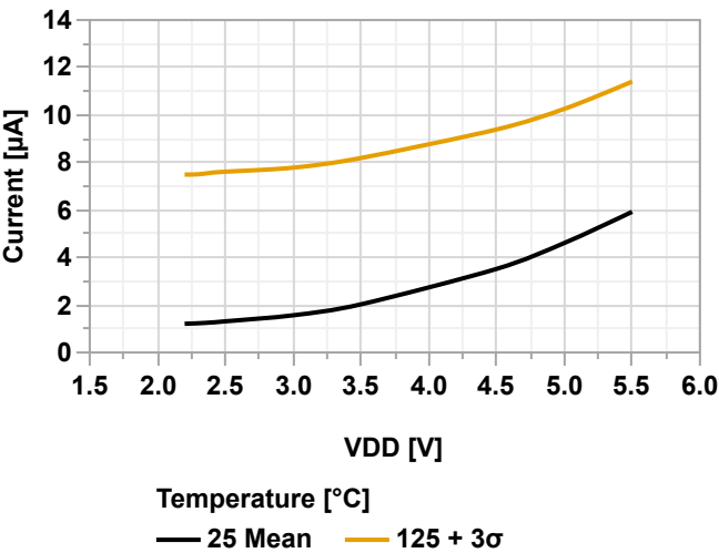
Figure 38-25. BOD Power Consumption vs. V_{DD} (BOD Sampling Mode @128 Hz)
