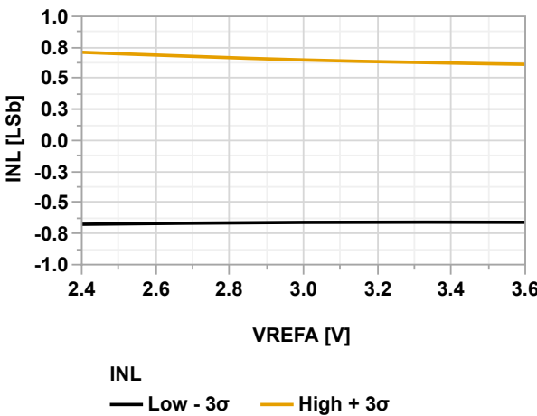
Figure 38-133. INL vs. V_{\text{REFA}} (ADC Differential Mode @60 kps, V_{\text{DD}} = 3.6\text{V} , T = 85^\circ\text{C} )
