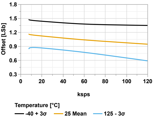
Figure 38-126. Offset Error vs. Sample Rate (ADC Differential Mode, V_{\text{REFA}} = V_{\text{DD}} = 3.6\text{V} )
