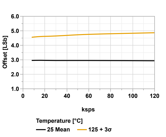
Figure 38-114. Offset Error vs. Sample Rate (ADC Single Ended Mode, V_{\text{REFA}} = V_{\text{DD}} = 3.0\text{V} )
