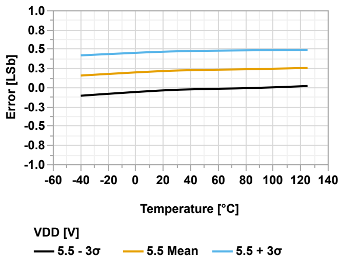
Figure 38-161. Offset Error vs. Temperature ( V_{\text{REFA}} = V_{\text{DD}} = 5.5\text{V} )
