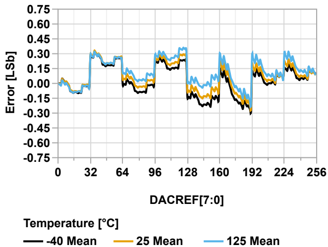
Figure 38-164. INL vs. DAC Code ( V_{\text{REFA}} = V_{\text{DD}} = 3.0\text{V} )
