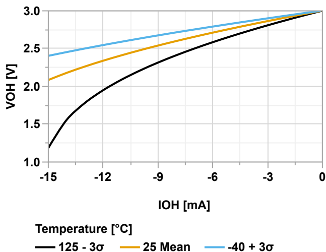
Figure 38-86. Output Pin - Minimum V_{OH} vs. Current, V_{DD} = 3.0V
