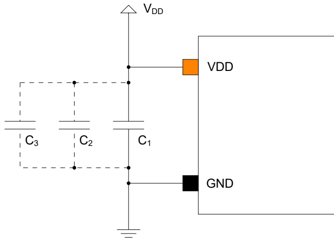
Figure 4-1. Recommended V DD Connection Circuit Schematic
