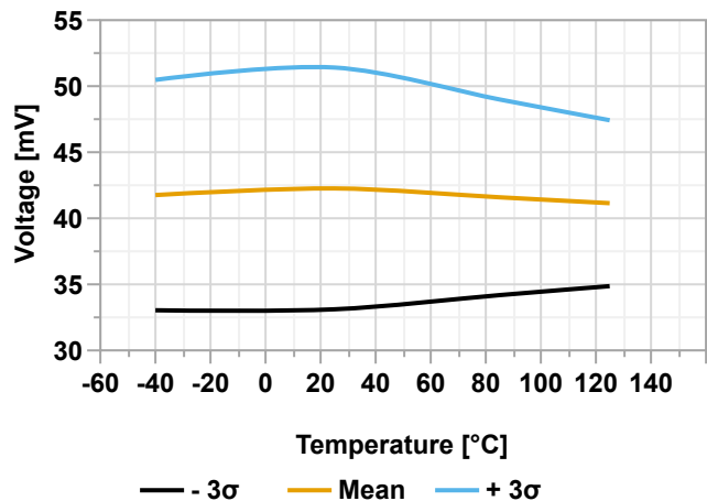
Figure 38-64. BOD Hysteresis vs. Temperature (BODCFG.LVL = 0x02)
