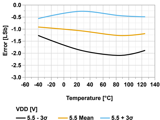
Figure 38-149. Gain Error vs. Temperature ( V_{REFA} = V_{DD} = 5.5V )
