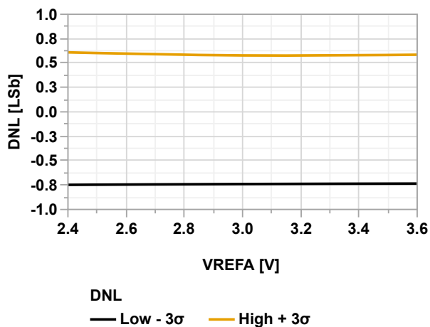
Figure 38-129. DNL vs. V_{\text{REFA}} (ADC Differential Mode @60 kps, V_{\text{DD}} = 3.6\text{V} , T = 85^\circ\text{C} )
