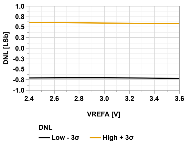
Figure 38-130. DNL vs. V_{\text{REFA}} (ADC Differential Mode @60 kps, V_{\text{DD}} = 3.6\text{V} , T = 125^\circ\text{C} )
