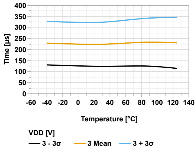
Figure 38-156. Settling Time vs. Temperature ( V_{\text{REFA}} = V_{\text{DD}} = 3.0\text{V} , Output Switch from 0x000 to 0x3FF)
