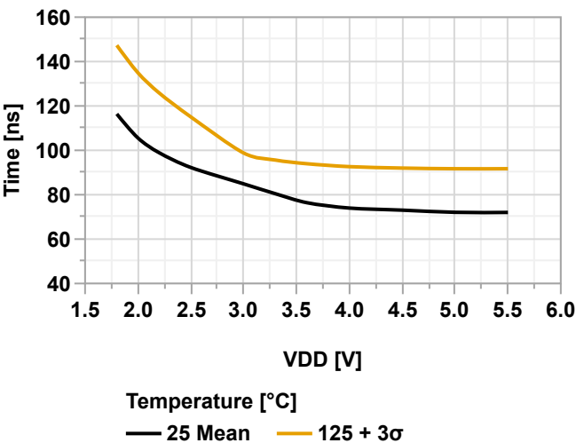
Figure 38-137. Rising Edge Response Time vs. V_{DD} ( V_{CM} = V_{DD}/2 , CTRLA.POWER = 0x00)
