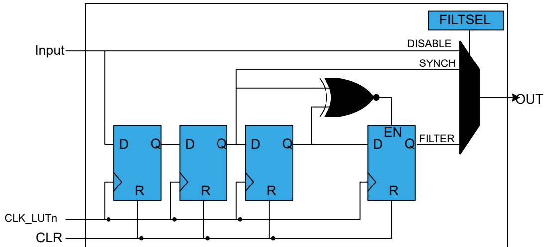
Figure 29-5. Filter
