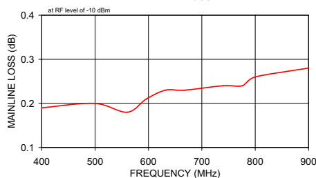
JDC-20-2 MAINLINE LOSS
