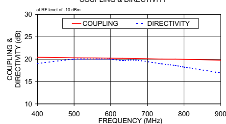
JDC-20-2 COUPLING & DIRECTIVITY
