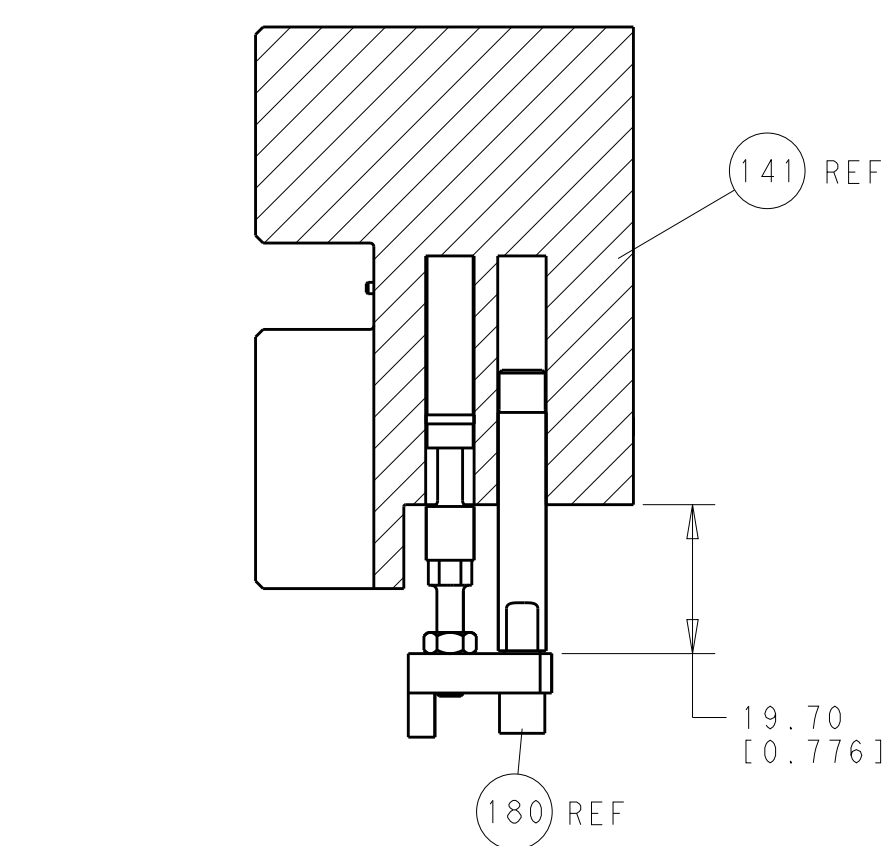
HOLDDOWN SET-UP
