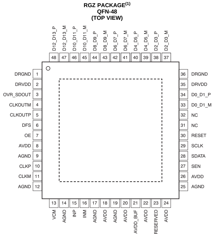
Figure 1. ADS41B49 LVDS Pinout
