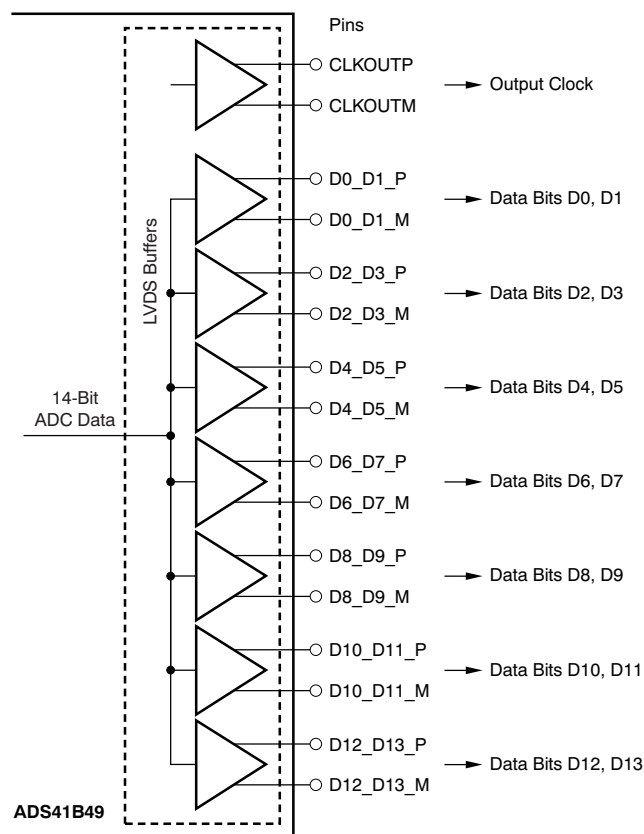
Figure 69. ADS41B49 LVDS Data Outputs
