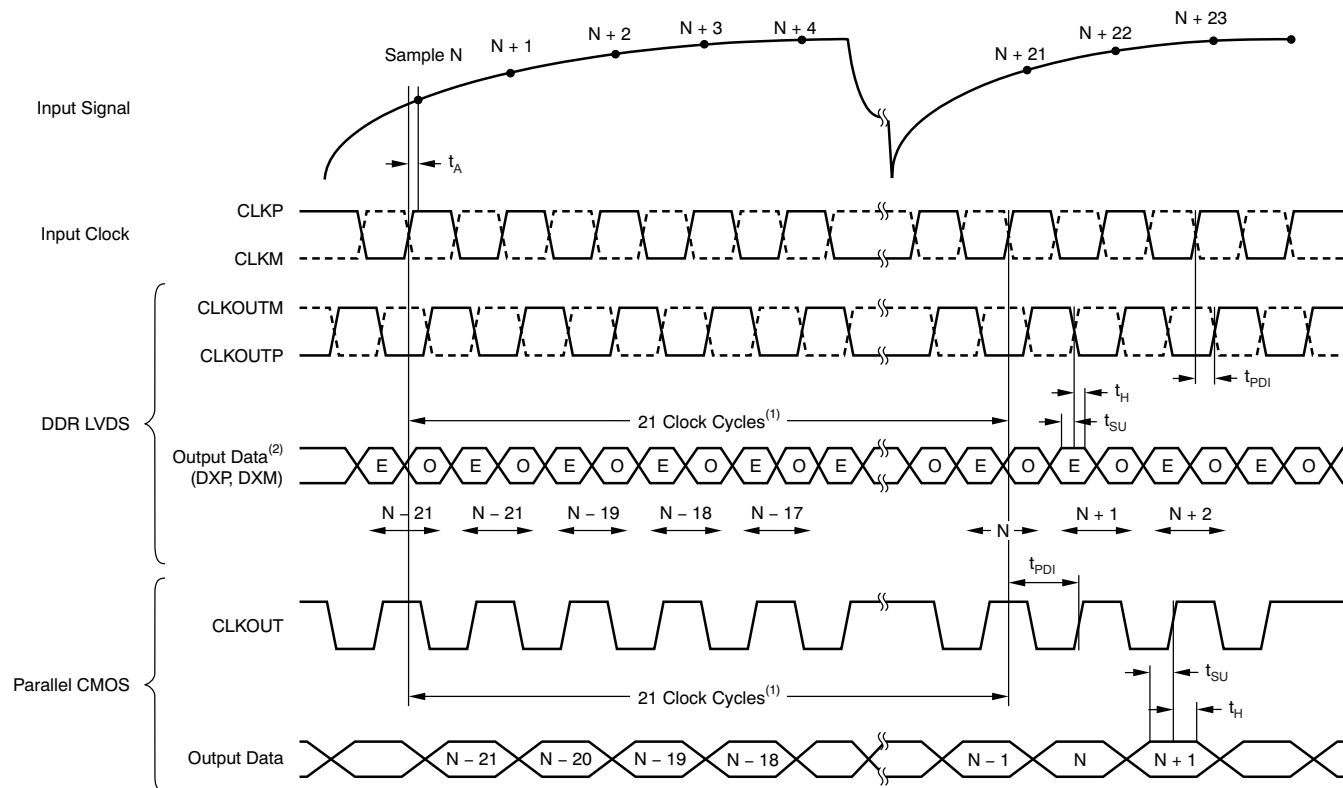
Figure 5. Latency Diagram
