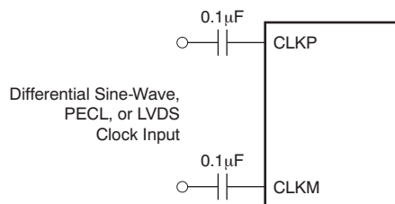
Figure 66. Differential Clock Driving Circuit
