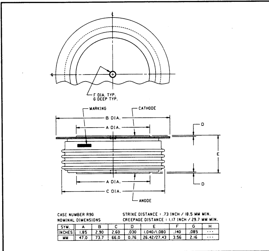
R9G2_12 Fast Recovery Rectifier 1200 Amperes Average, 3600 Volts
