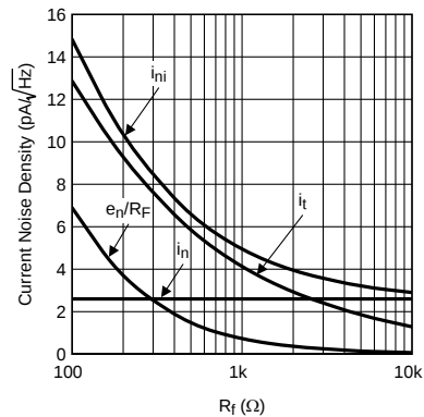
Figure 59. Current Noise Density vs. Feedback Resistance
