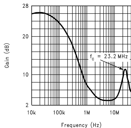
Figure 55. Equalizer Frequency Response
