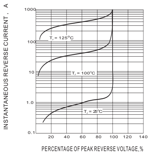
Fig.5-TYPICAL REVERSE CHARACTERISTIC
