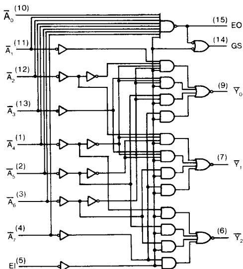
Fig. 1 Logic diagram
