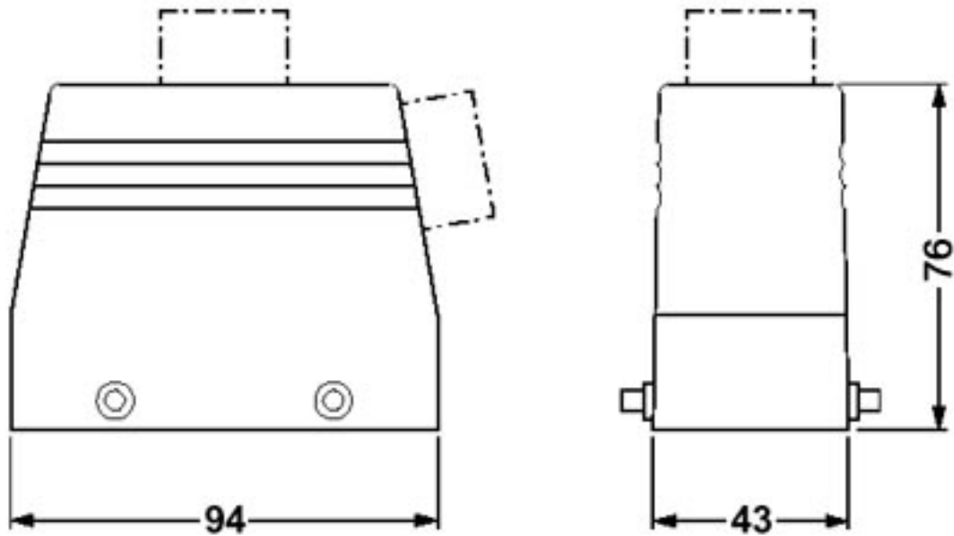
Dimensioned drawing
