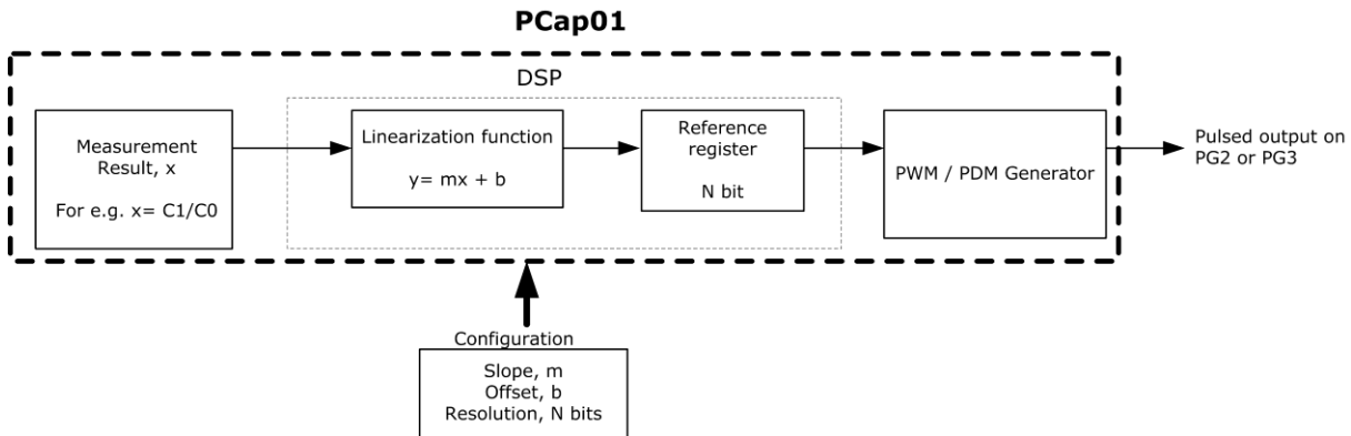
Figure 4-7: Pulse generation
