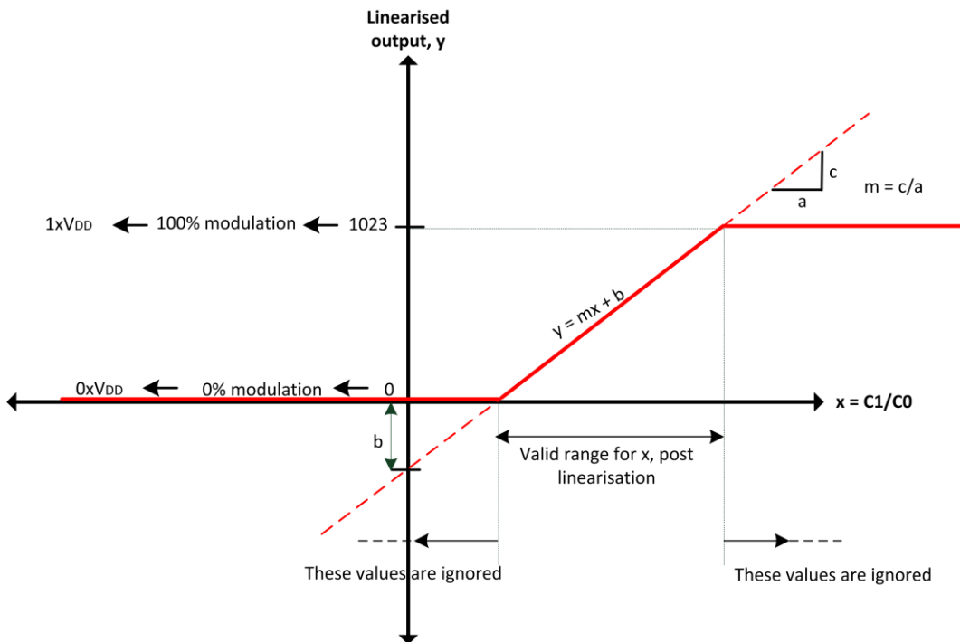
Figure 4-8: PWM-PDM linearization
