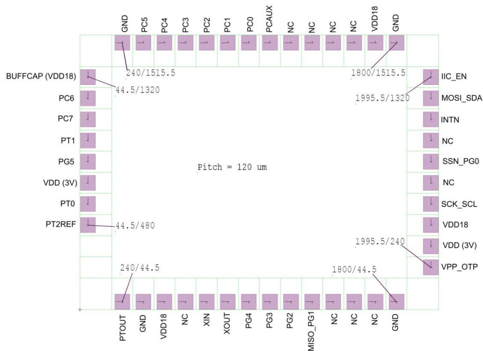
Figure 2-11: Pad Layout
