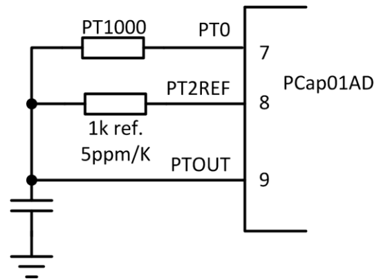
Figure 3-14 RDC with external resistors
