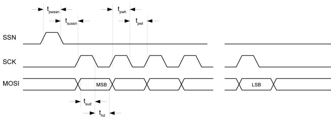
Figure 4-4: SPI Write
