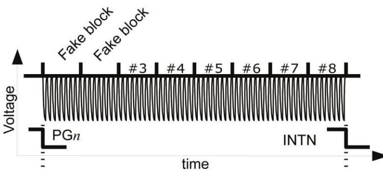
Figure 3-4 Measurement cycle
