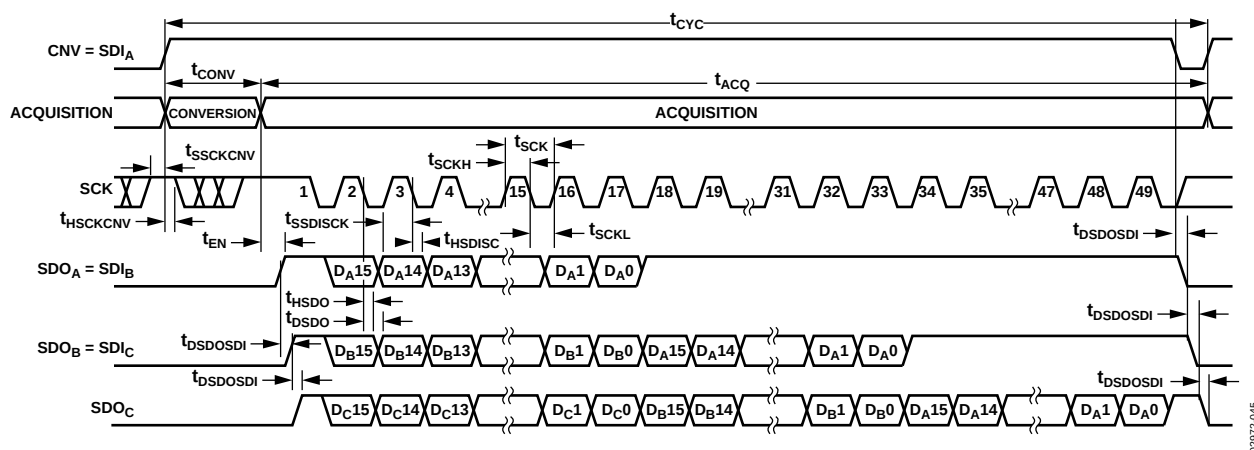
Figure 45. Chain Mode with BUSY Indicator Serial Interface Timing
