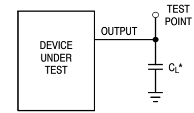
Figure 4. Test Circuit
