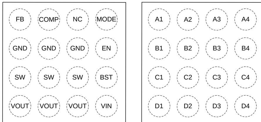
YKB Package 16-Pin DSBGA Top View
