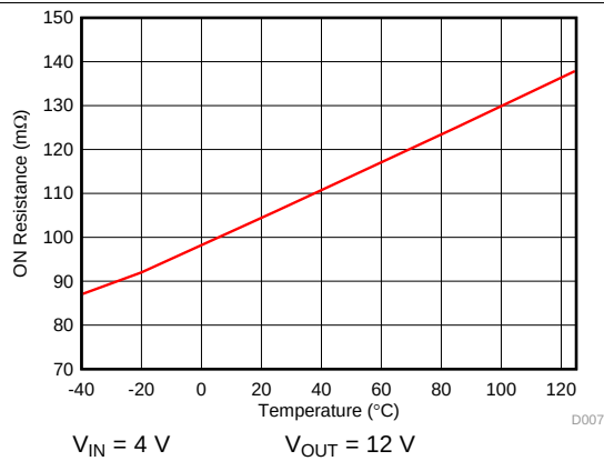
Figure 7. High-side R_{DS(ON)} vs Temperature
