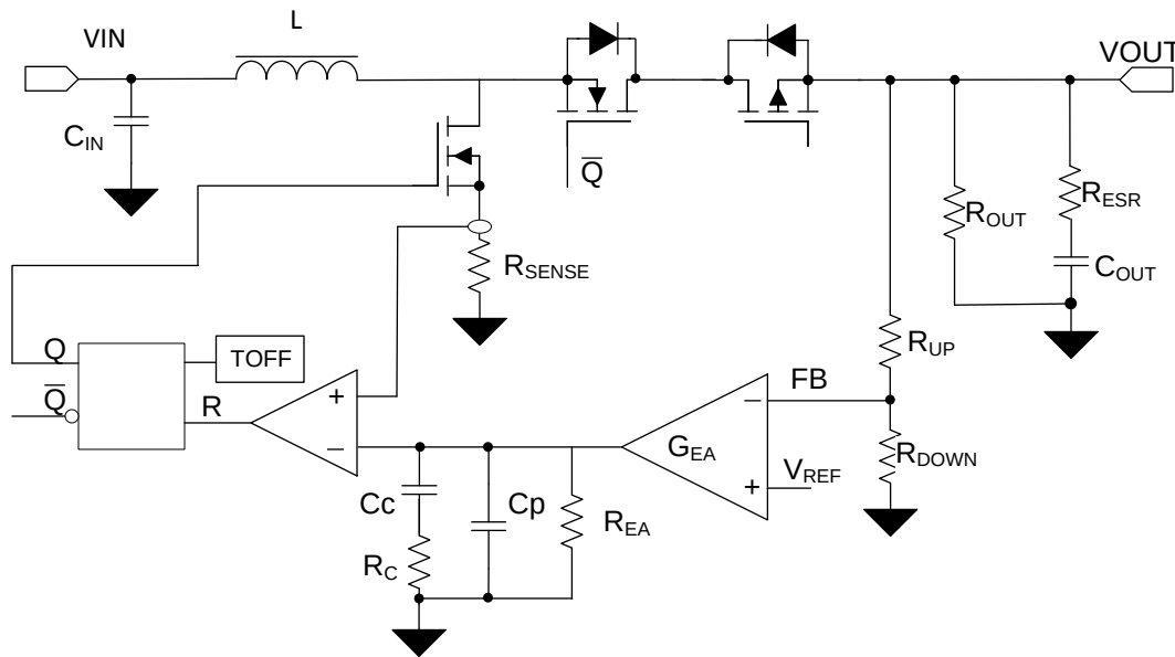
Figure 11. TPS61372 Control Equivalent Circuitry Model
