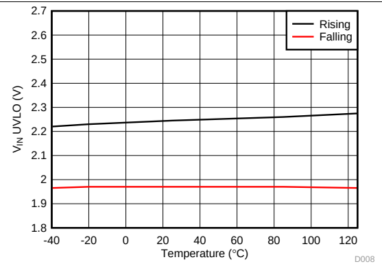
Figure 8. UVLO Threshold vs Temperature
