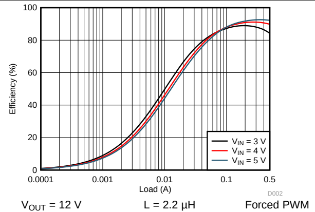
Figure 2. Efficiency vs Load
