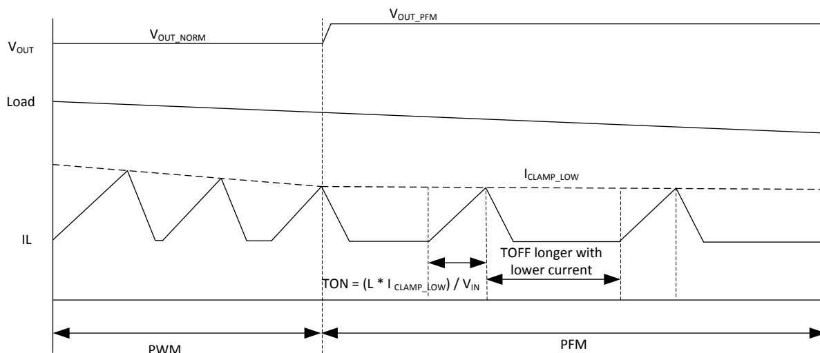
Figure 9. Auto PFM Operation Behavior
