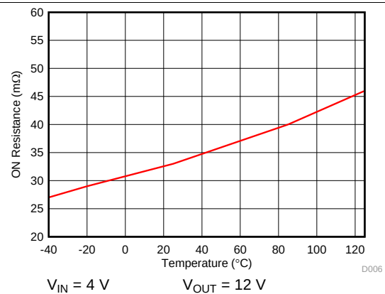
Figure 6. Low-Side R_{DS(on)} vs Temperature
