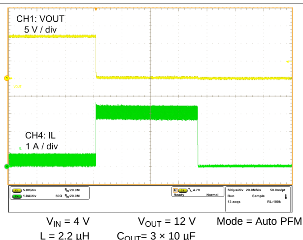
Figure 17. Shorted Output
