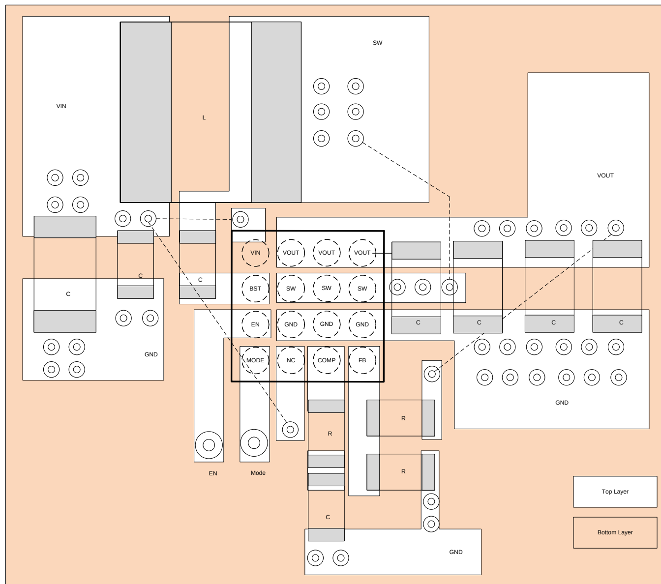
Figure 18. Recommended Layout
