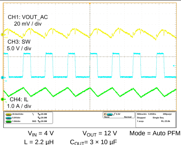
Figure 12. Steady-State at 200 mA Load
