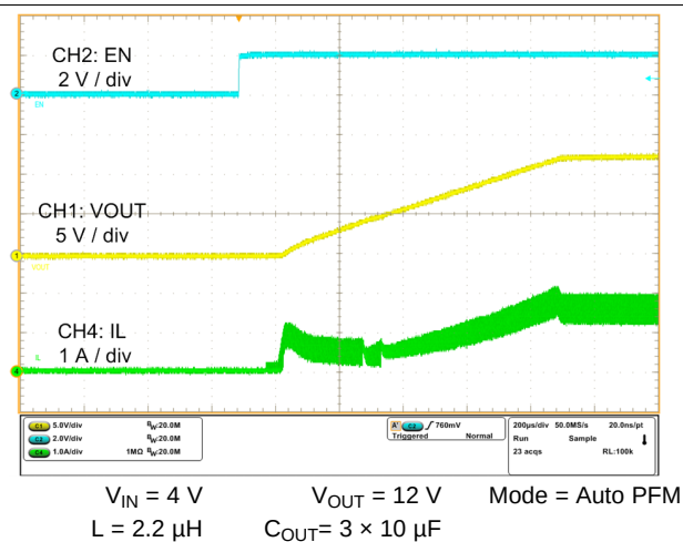
Figure 14. Start-Up by EN, Load = 12.5 Ω
