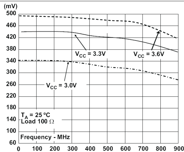
Figure 3. LVPECL Output Swing Vs Frequency
