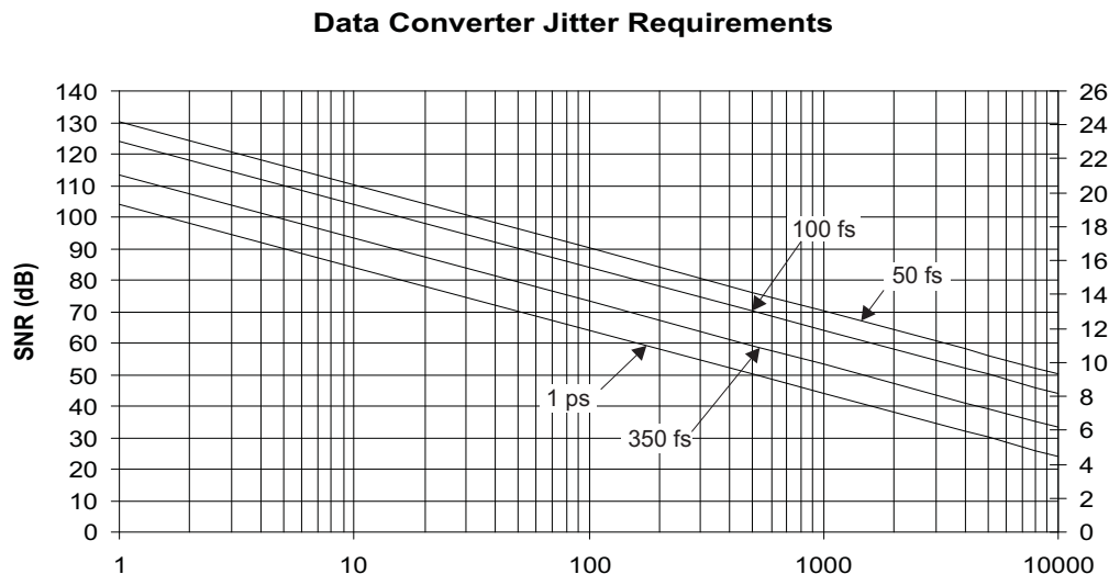
Figure 37. Data Converter Jitter Requirements
