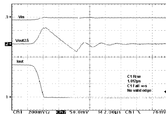
Figure 22 : Load Transient
