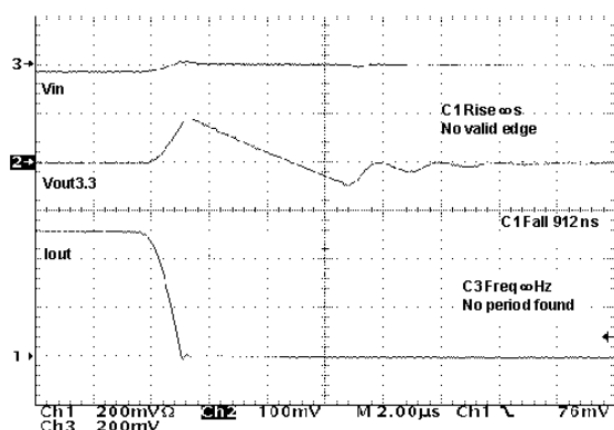
Figure 21 : Load Transient
