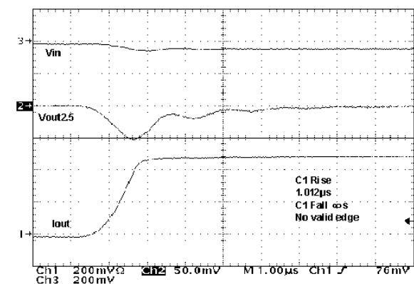
Figure 23 : Load Transient
