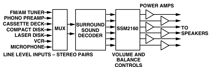
Figure 5. Typical Signal Chain Using the SSM2160
