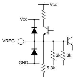
31pin (36pin)
