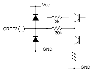
27pin (32pin)
