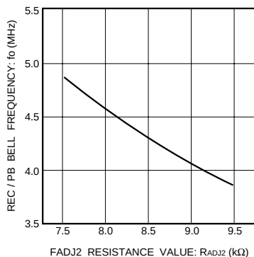
Fig. 10 REC / PB BELL fo frequency adjustment range
