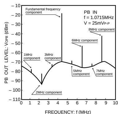
Fig. 14 PB OUT spurious characteristics
