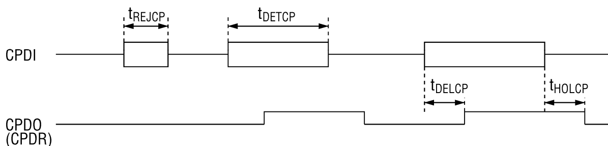
Figure 1 CPT Detect Timing
