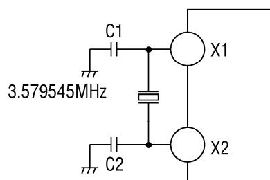
Figure 6 Crystal Connection
