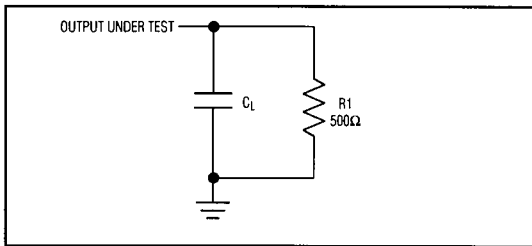
Figure 7. Receiver Enable/Disable Test Circuit 2
