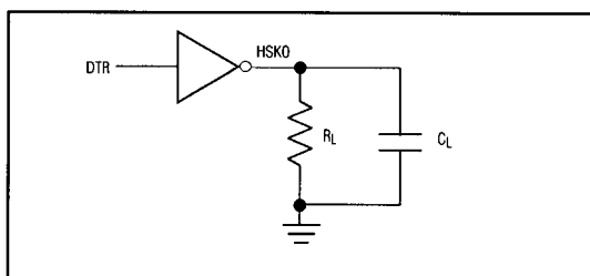
Figure 5. Single-Ended Driver Timing Test Circuit
