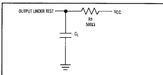
Figure 6. Receiver Enable/Disable Test Circuit 1
