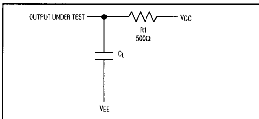
Figure 3. Driver Enable/Disable Test Circuit 1
