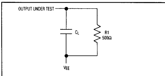
Figure 4. Driver Enable/Disable Test Circuit 2
