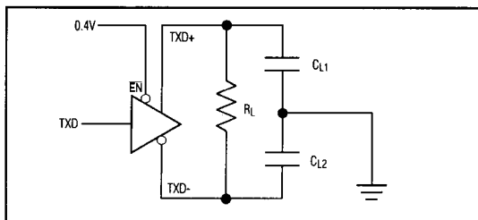
Figure 2. Differential Driver Timing Test Circuit
