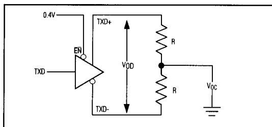
Figure 1. Differential and Common-Mode Output Voltages
