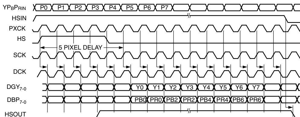
Figure 10. YPBPR422 Mode
