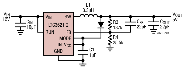
5V OUT with 400mA Burst Mode Operation, 2.25MHz
