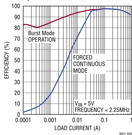
Efficiency vs Load at Dropout Operation
