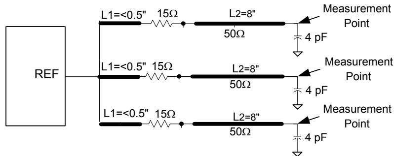
Figure 3. Single-ended REF Triple Load Configuration
