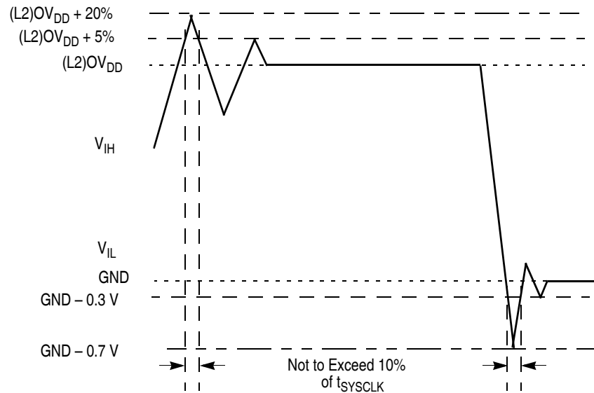
Figure 2. Overshoot/Undershoot Voltage
