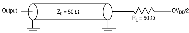
Figure 11. AC Test Load for the JTAG Interface
