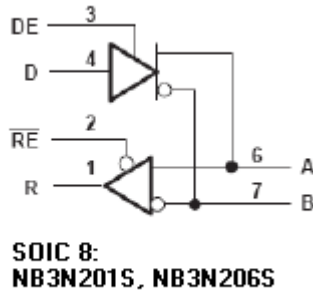
Figure 1. Logic Diagram
