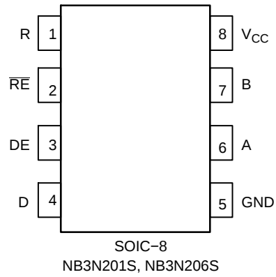
Figure 2. Pinout Diagram (Top View)
