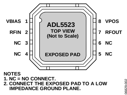
Figure 2. Pin Configuration
