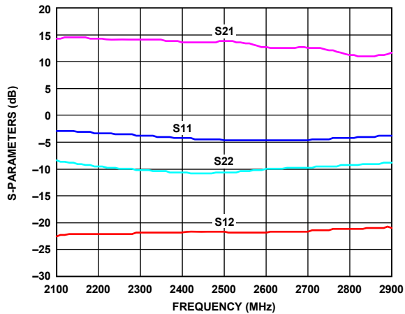
Figure 39. Typical S-Parameters, Log Magnitude
