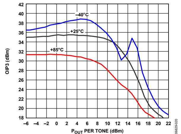
Figure 20. OIP3 vs. Output Power (P OUT ) and Temperature
