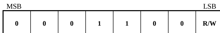
Figure 10.4. Slave Address
