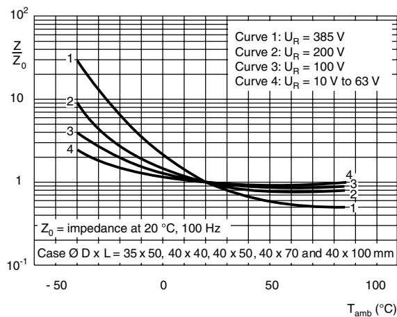
Fig.16 Typical multiplier of impedance as a function of ambient temperature.
