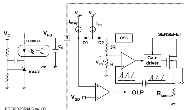
Figure 21. Pulse-Width-Modulation Circuit
