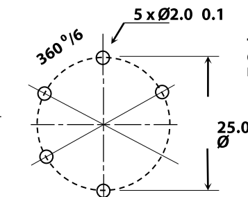
PC Board Mounting Holes
