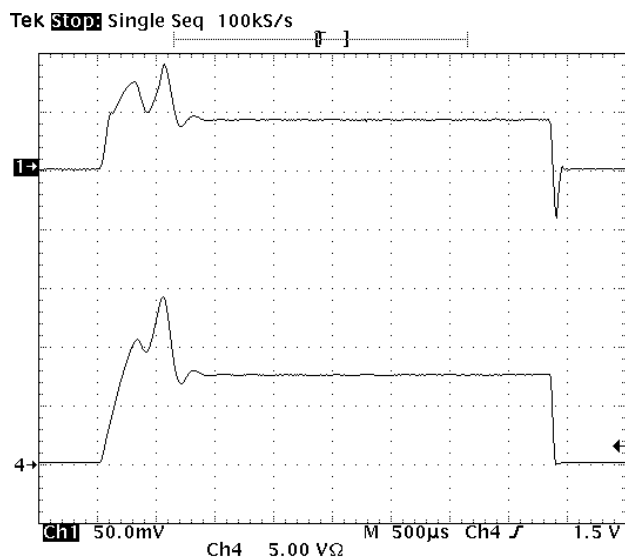
Figure 7 - Output Shorted at start-up.
