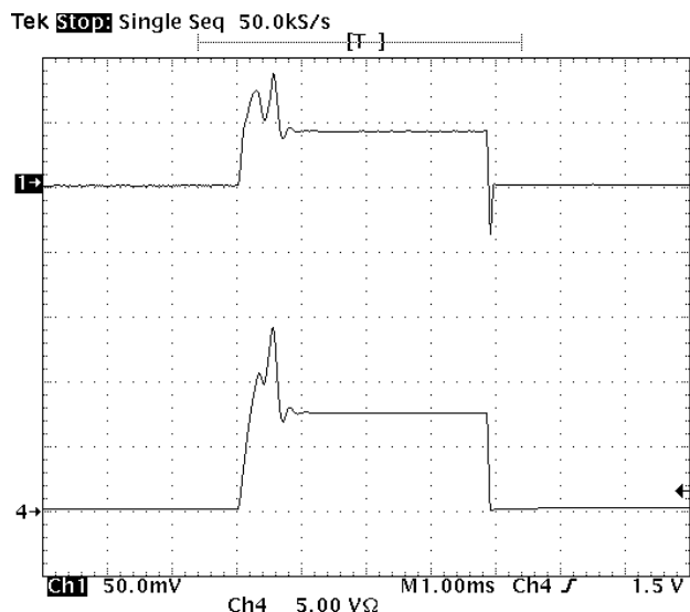
Figure 6 - Output Shorted at start-up.
