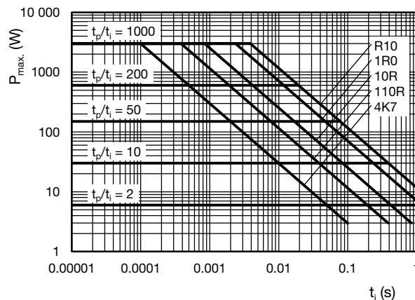
AC03 Pulse on a regular basis; maximum permissible peak pulse power ( \hat{P}_{max.} ) as a function of pulse duration ( t_i )
