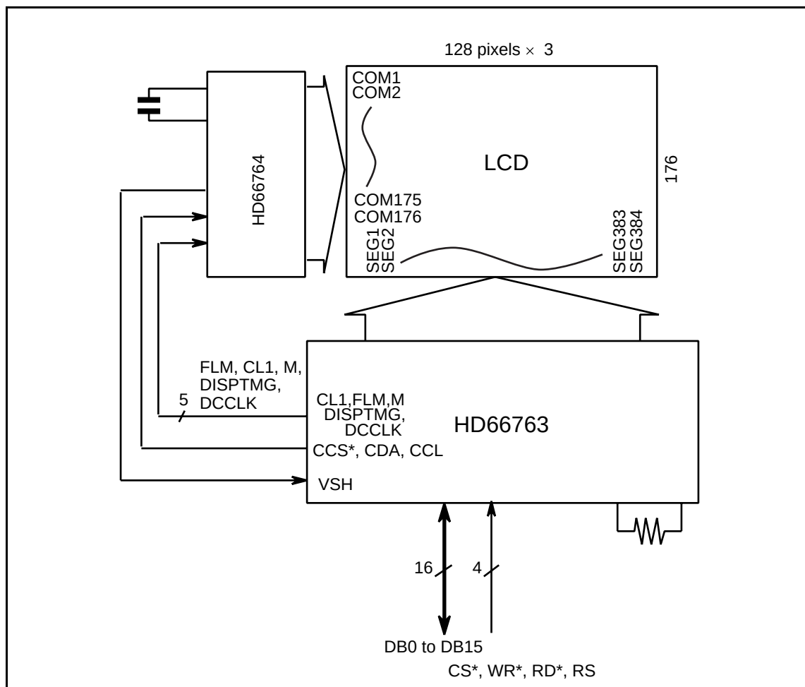
Figure 8 System Configuration
