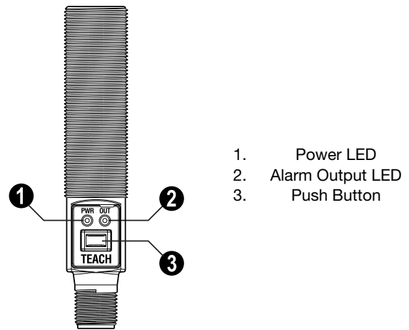
Figure 1. Sensor Features
