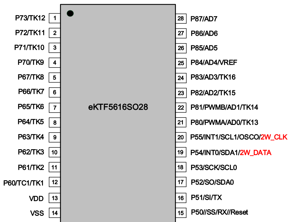
Figure 3-1 SOP-28 Pin Assignment
