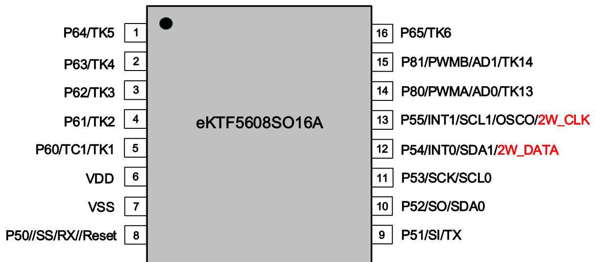
Figure 3-4 SOP-16A Pin Assignment
