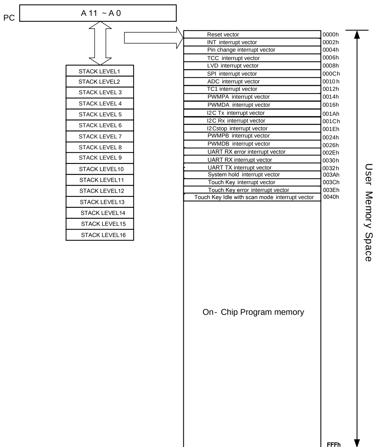
Figure 6-1 eKTF5616/08 Program Counter Organization
