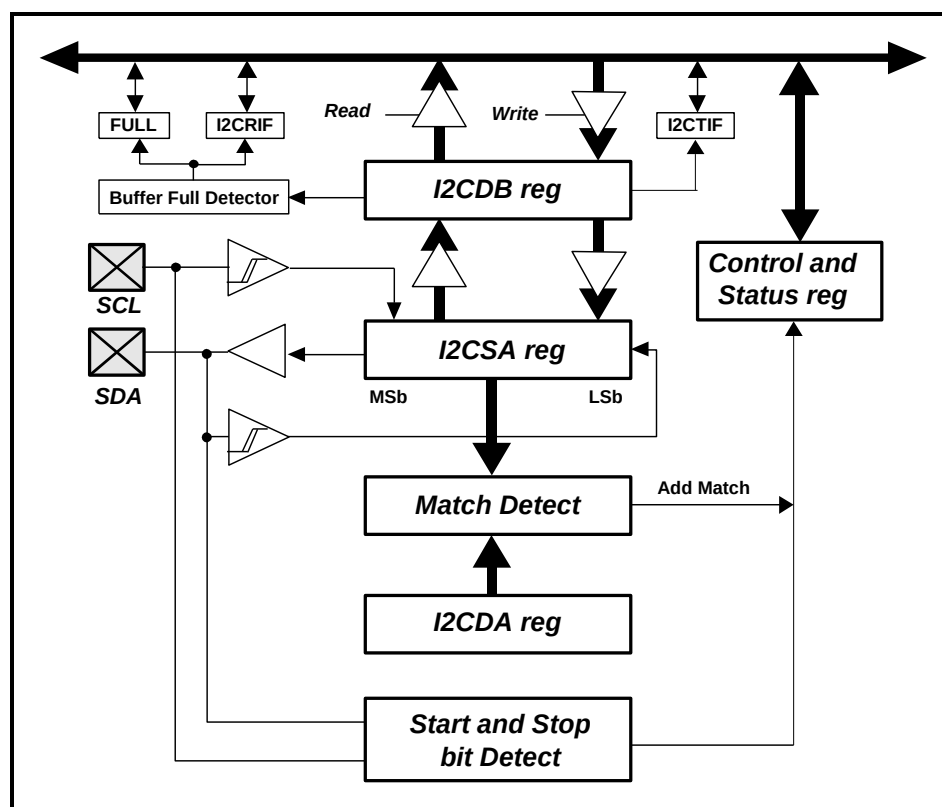
Figure 6-11 eKTF5616/08 I²C Block Diagram
