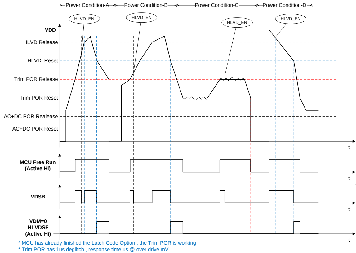
Figure 1.HLVD waveform situation
