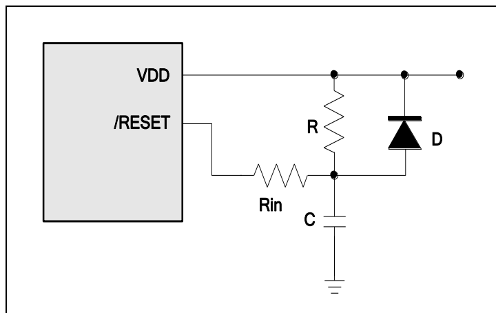
Figure 6-15 External Power-Up Reset Circuit
