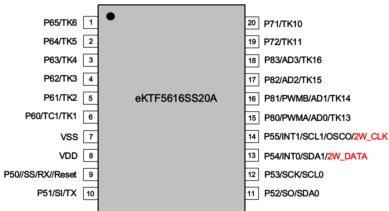
Figure 3-5 SSOP-20A Pin Assignment
