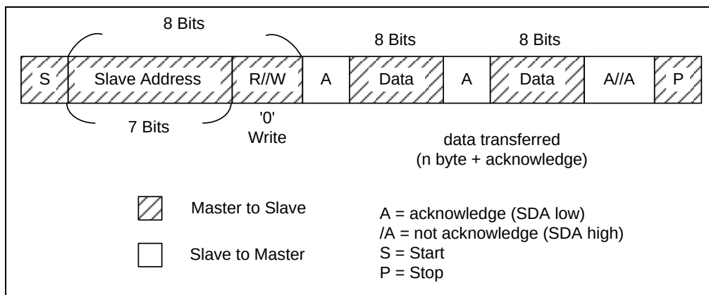
Figure 6-13a Master-Transmitter Transmits to Slave-Receiver with 7-Bit Slave Address
