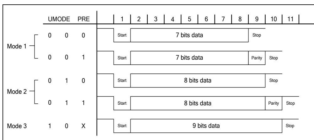
Figure 6-18a UART Model
