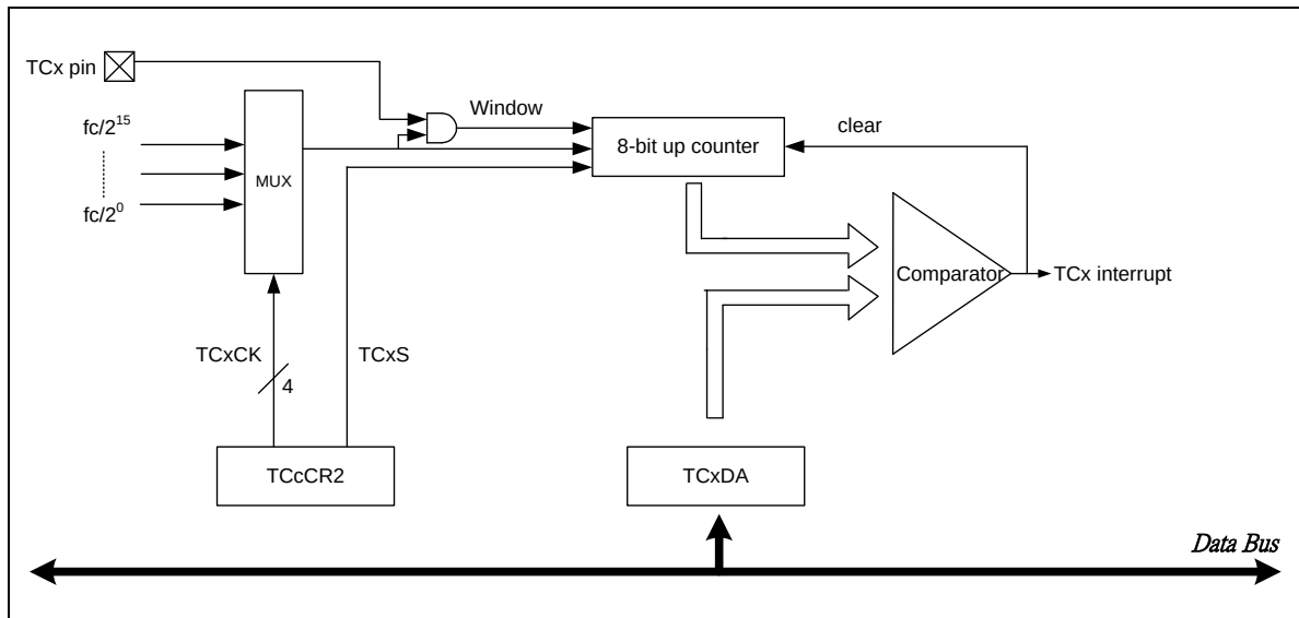
Figure 6-13a Window Mode Block Diagram
