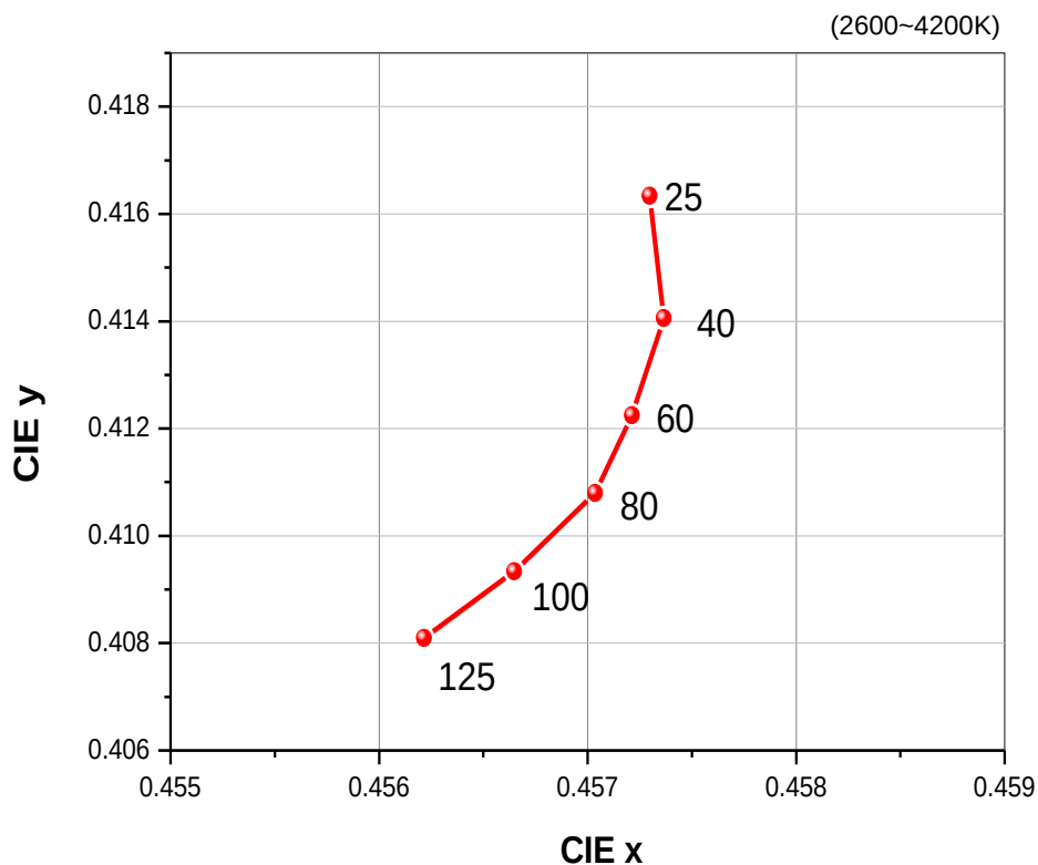
Fig 8. Chromaticity Coordinate vs. Junction Temperature, I_F=65\text{mA}
