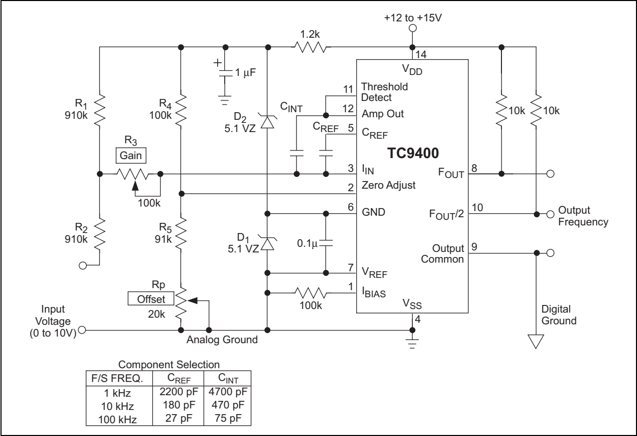
FIGURE 5-2: Voltage-to-Frequency
