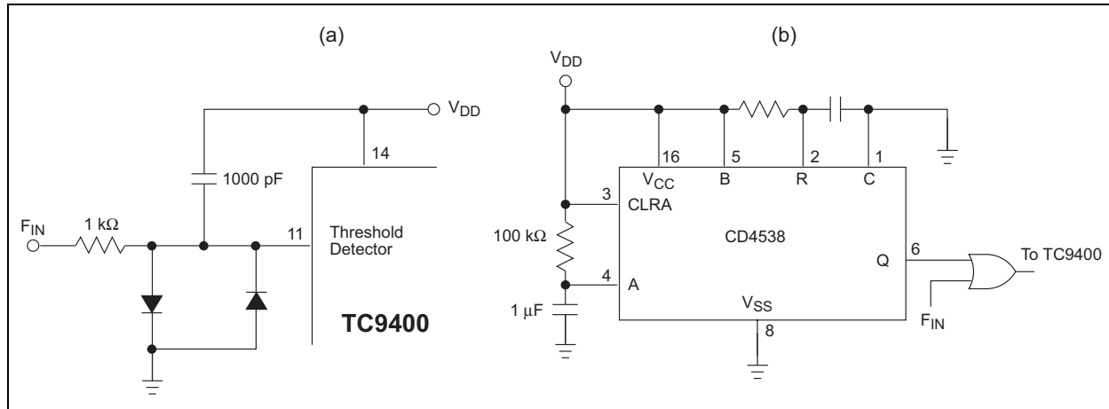
FIGURE 8-1: Power-On Operation/Reset
