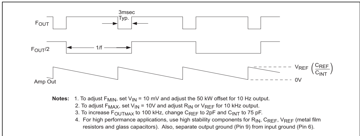
FIGURE 4-1: Output Waveforms
