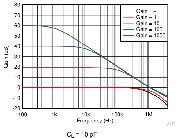
Figure 6-6. Closed-Loop Gain vs Frequency
