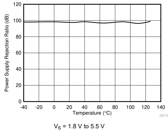
Figure 6-9. DC PSRR vs Temperature
