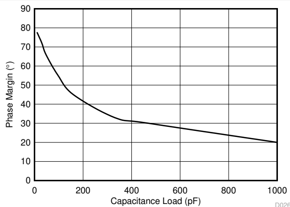
Figure 6-21. Phase Margin vs Capacitive Load
