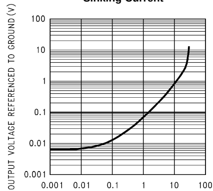
Output Characteristics Sinking Current
