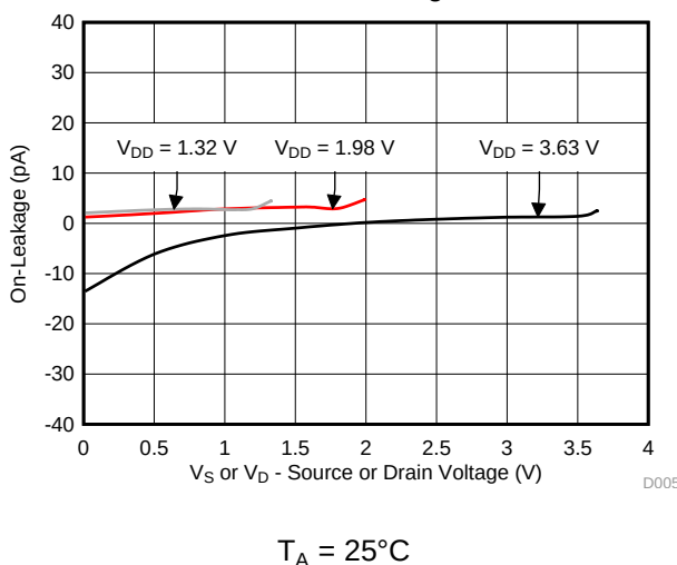
Figure 33. On-Leakage vs Source or Drain Voltage
