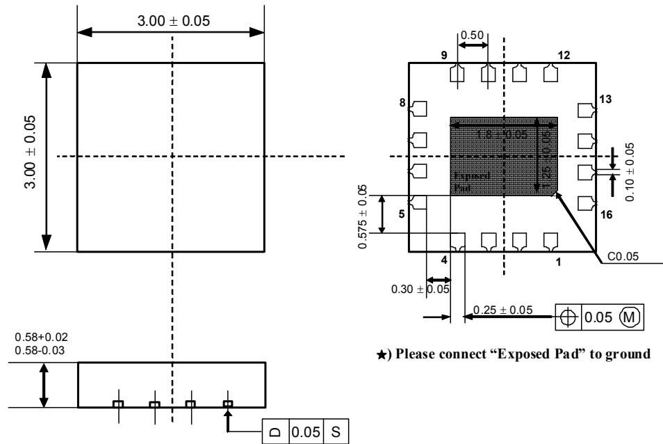
Figure 3 Package Information
