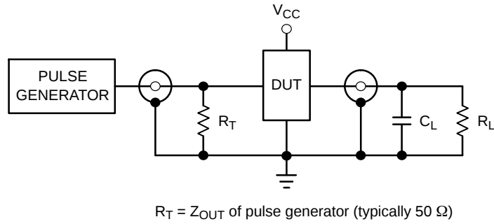
Figure 4. Test Circuit
